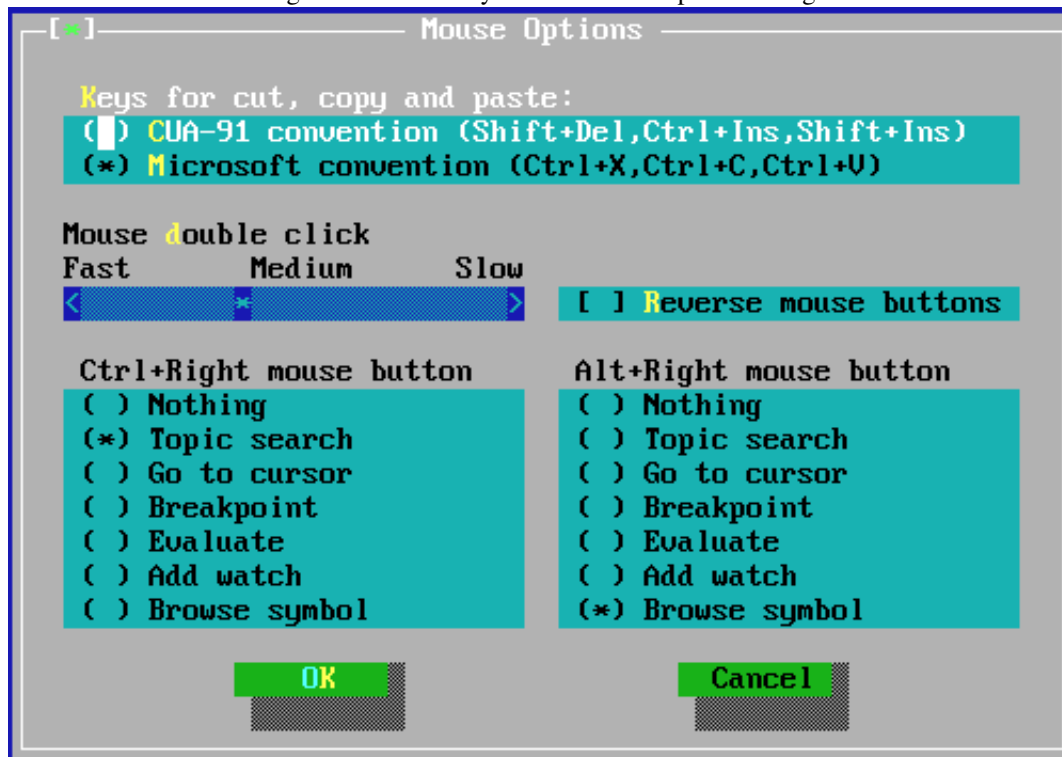
Figure 6.36: The Keyboard &amp; mouse options dialog
